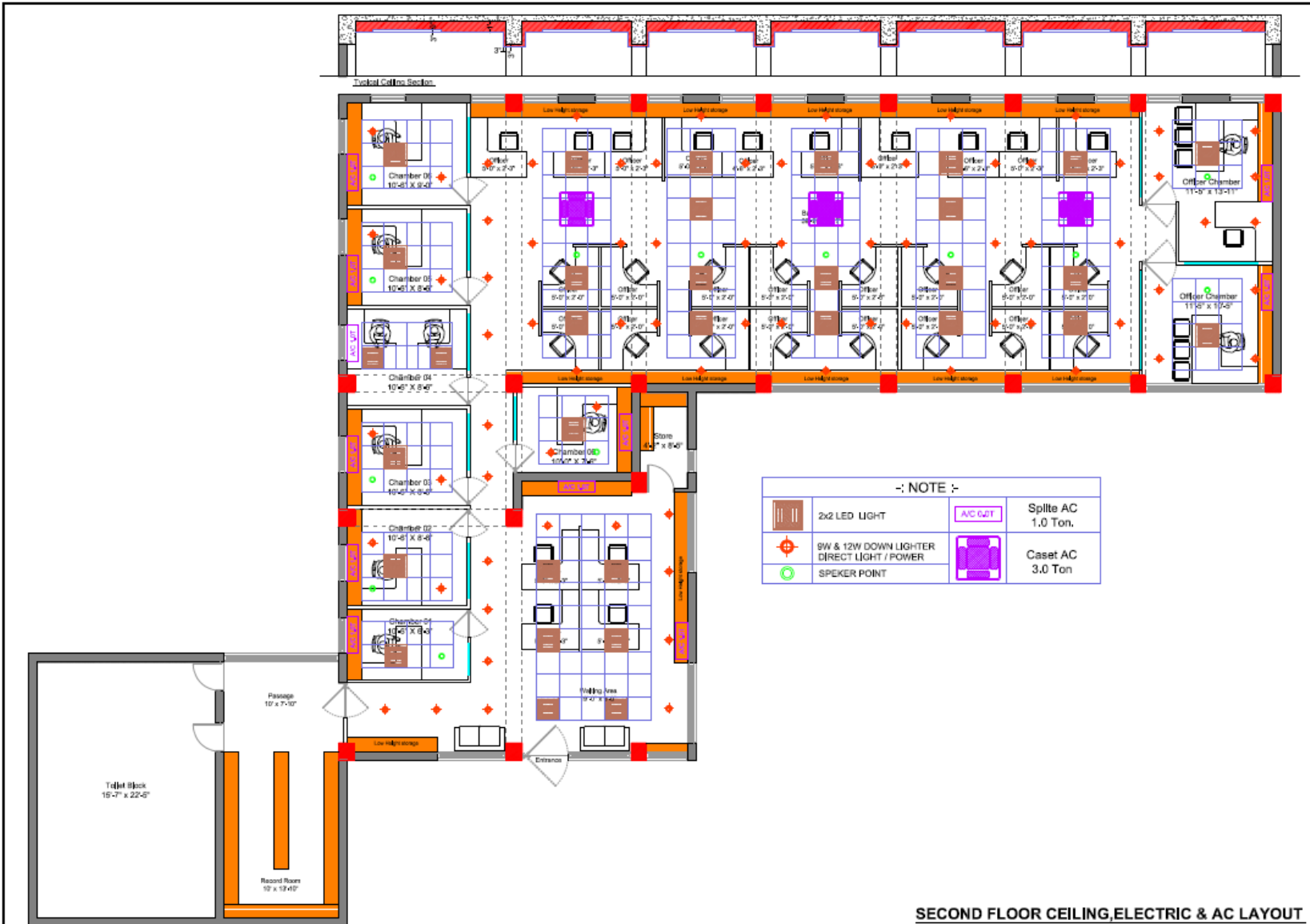
SECOND FLOOR CEILING, ELECTRIC & AC LAYOUT
